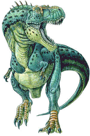
Tyrannosaurus rex
